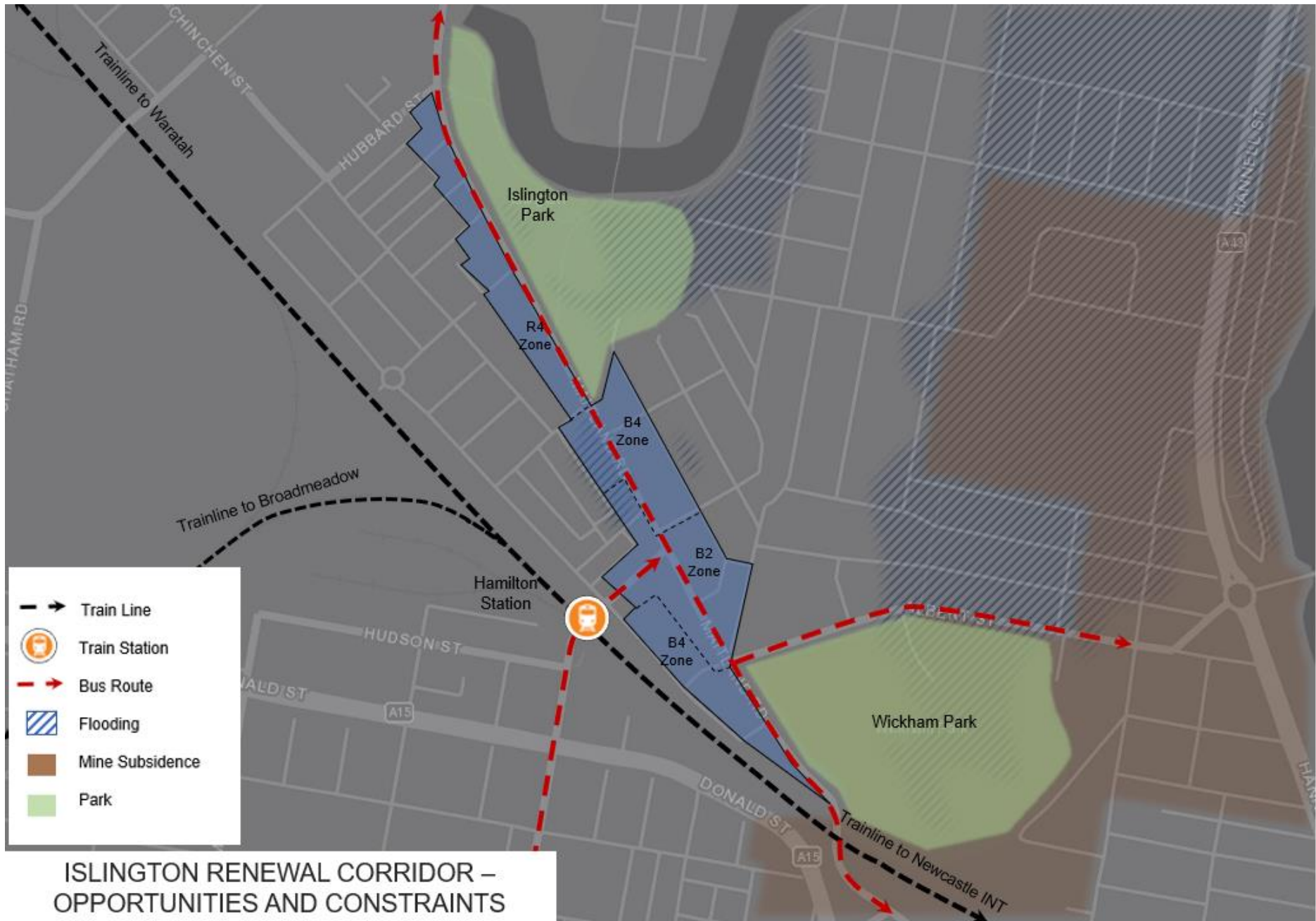
Figure 4. Opportunities and constraints of the Islington Urban Renewal Corridor
